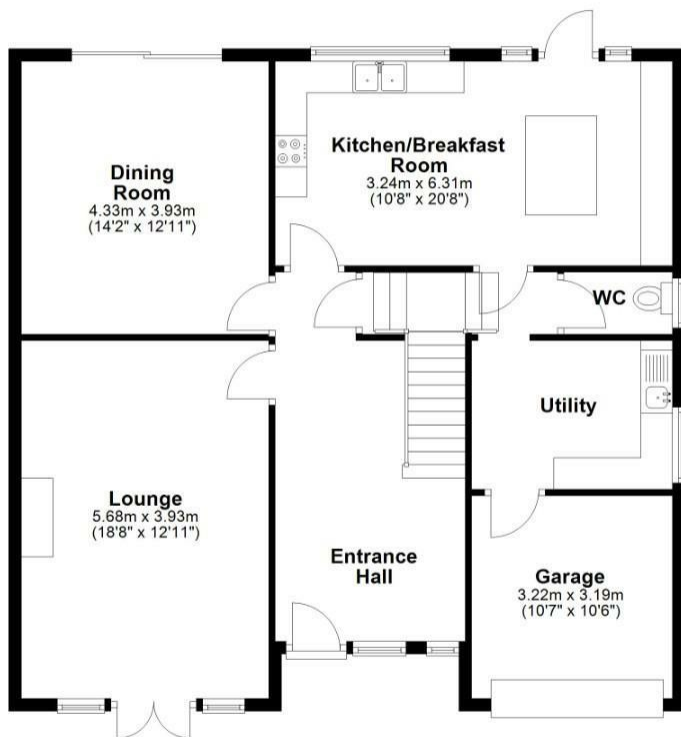
Ground Floor Approx. 101.5 sq. metres (1092.1 sq. feet)
